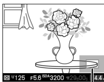
Navigation window
